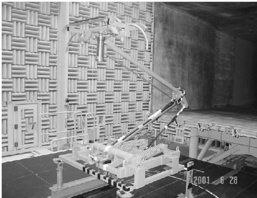
Fig. 4 Pantograph of KHST under wind tunnel test
