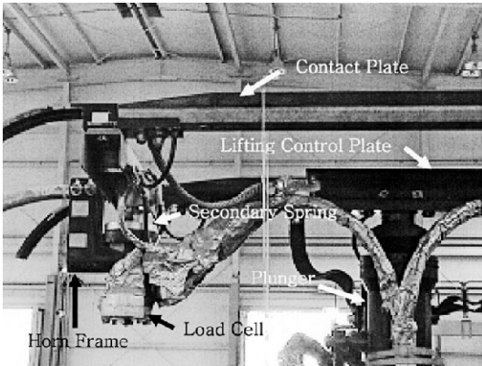
Fig. 2 Details of pantograph
