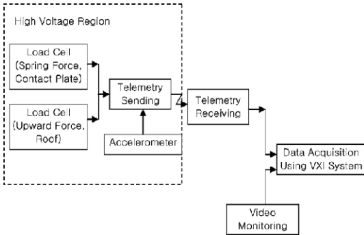
Fig. 7 Configuration of contact force measuring system
