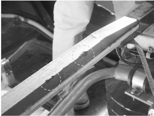
Fig. 17 Damaged carbon strip of contact plate after strong arc generation
