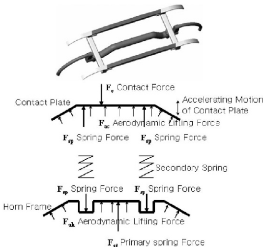
Fig. 3 Forces acting on pantograph
